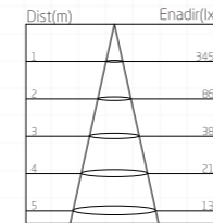
100W-Lux Distance Curve
