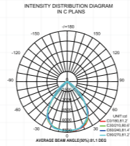
100W-Light Distribution Curve
